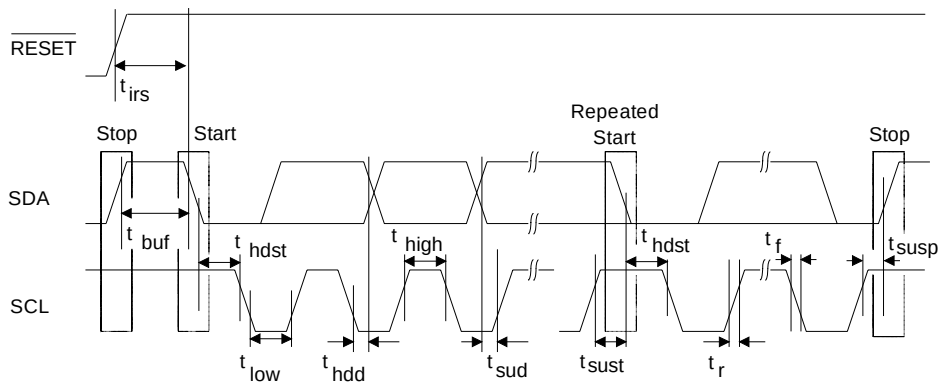
Figure 7. I²C Control Port Timing
