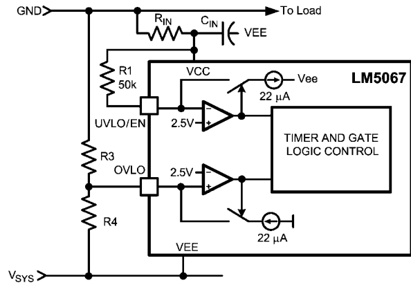
FIGURE 13. UVLO = POR_{EN}
