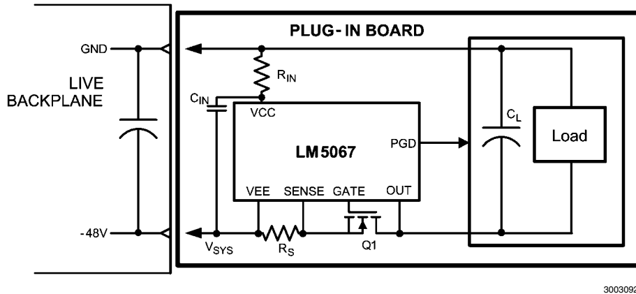
FIGURE 2. LM5067 Application
