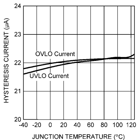
UVLO &amp; OVLO Hysteresis Current vs. Temperature
