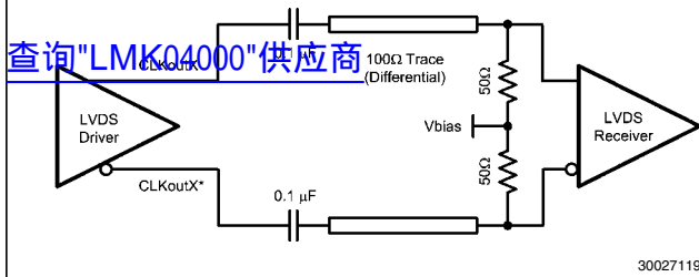
FIGURE 11. Differential LVDS Operation, AC Coupling, External Biasing at the Receiver
