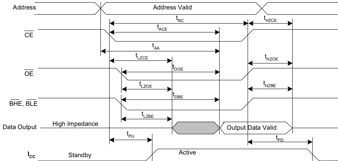
Figure 7. SRAM Read Cycle #2: \overline{\text{CE}} and \overline{\text{OE}} Controlled [3, 14, 18]
