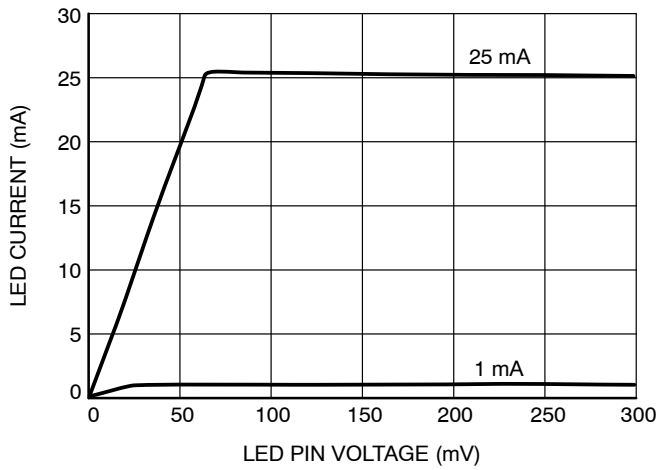
Figure 9. Dropout Characteristics
