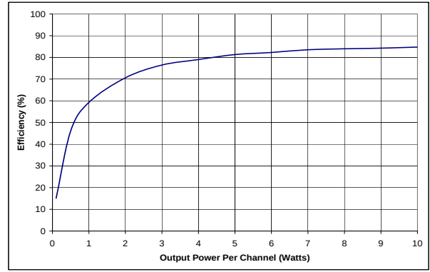
Figure 24. Efficiency ( R_L = 6\ \Omega )
