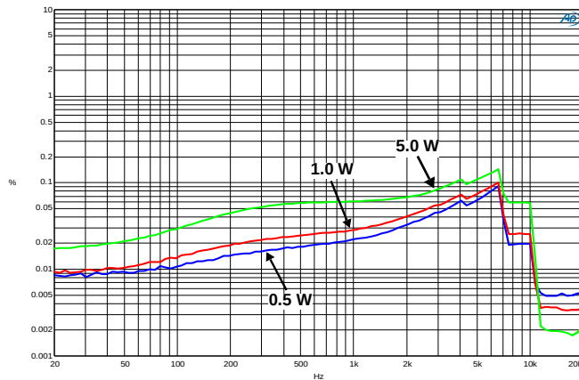
Figure 13. THD+N vs. Frequency ( R_L = 8 \Omega )
