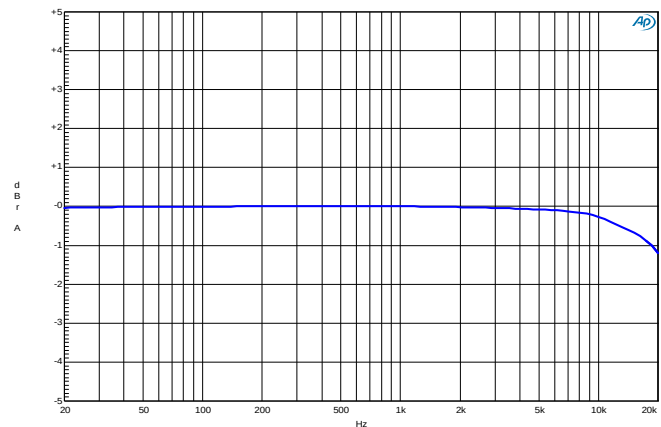
Figure 16. Frequency Response ( P_{OUT} = 1 \text{ W} , R_L = 6 \Omega )
