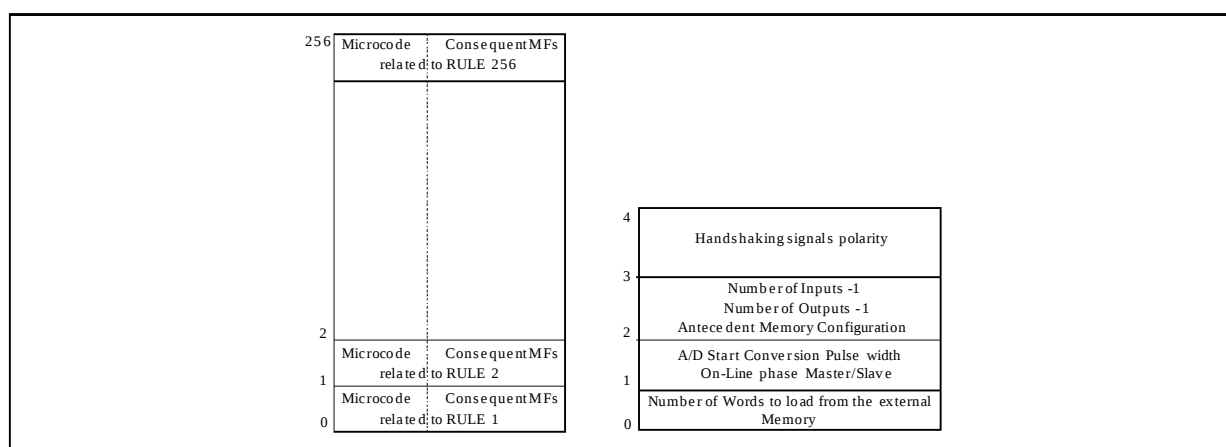
Figure 13. Program/Consequent Memory and Register Bench.
