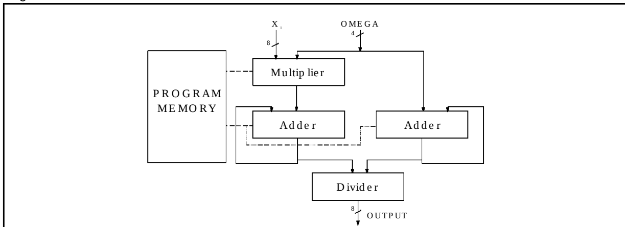
Figure 10. Defuzzifier Structure.
