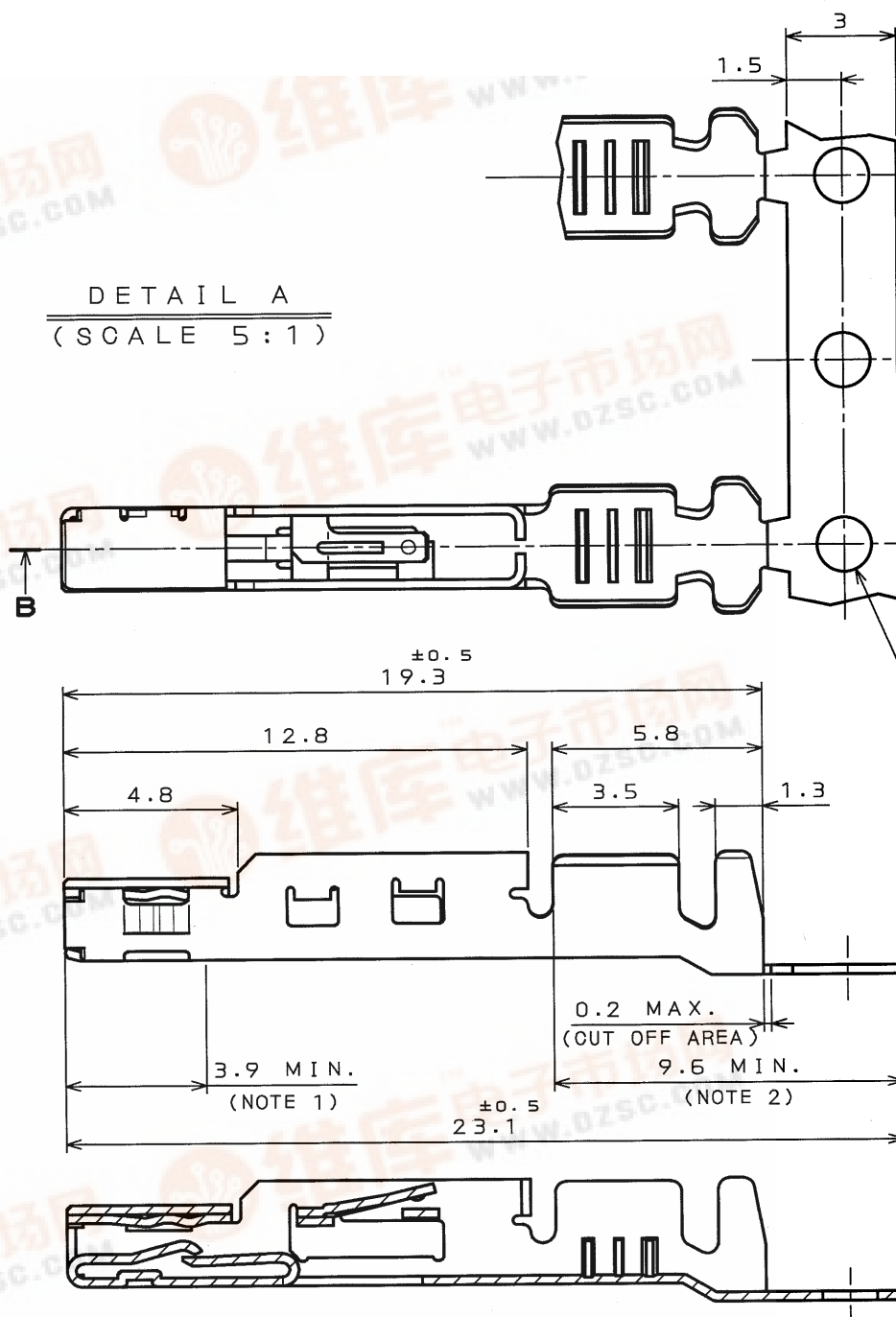
SECT. B-B (SCALE 5:1)
