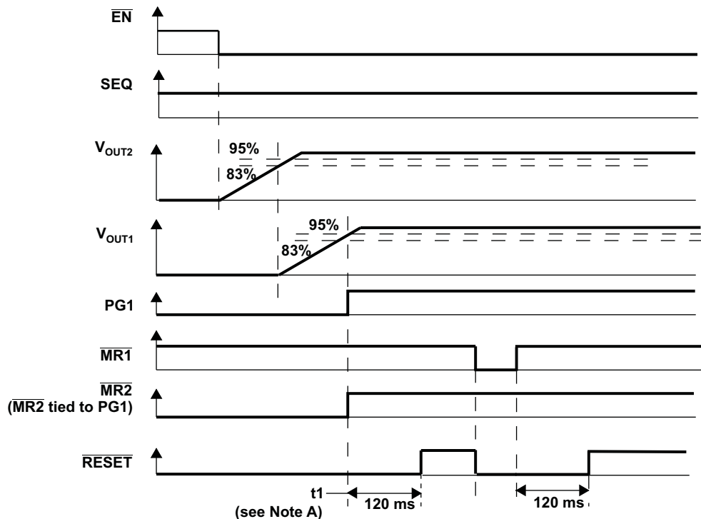
Figure 35. Timing When MR1 Is Toggled
