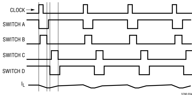
(4a) Buck-Boost Mode ( V_{IN} \geq V_{OUT} )
