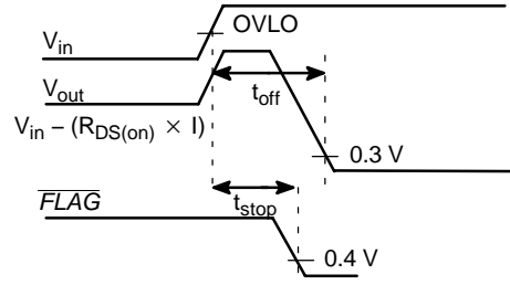
Figure 4. Shutdown on Overvoltage Detection
