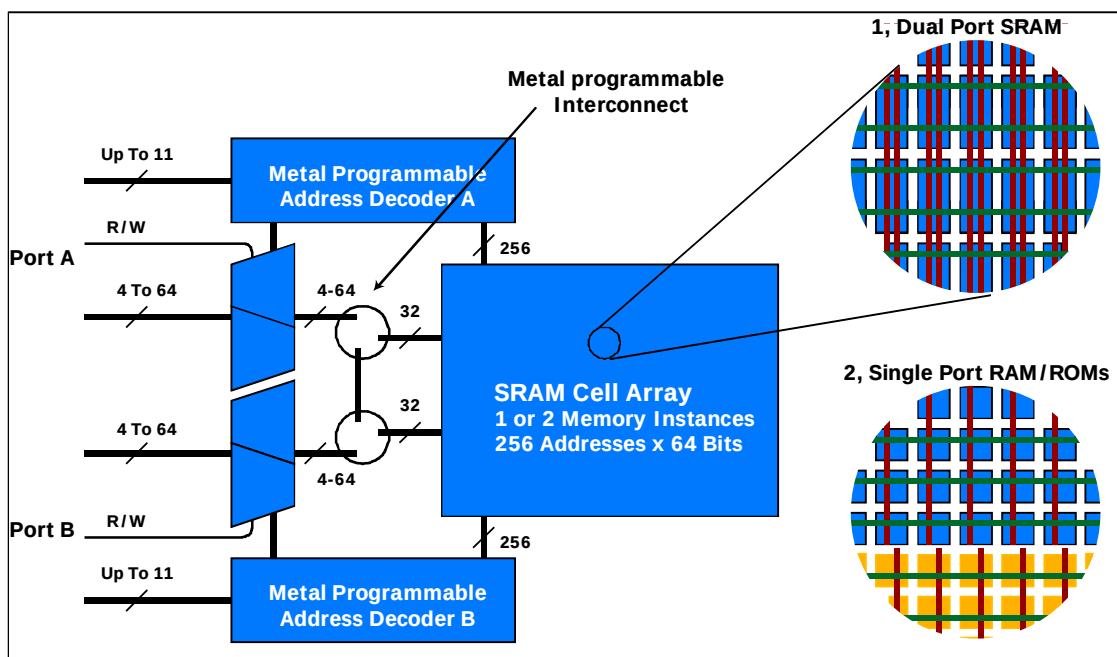
Figure 1. CX5000 CX-Memory Configurations
