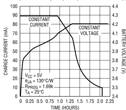
Complete Charge Cycle (130mAh Battery)
