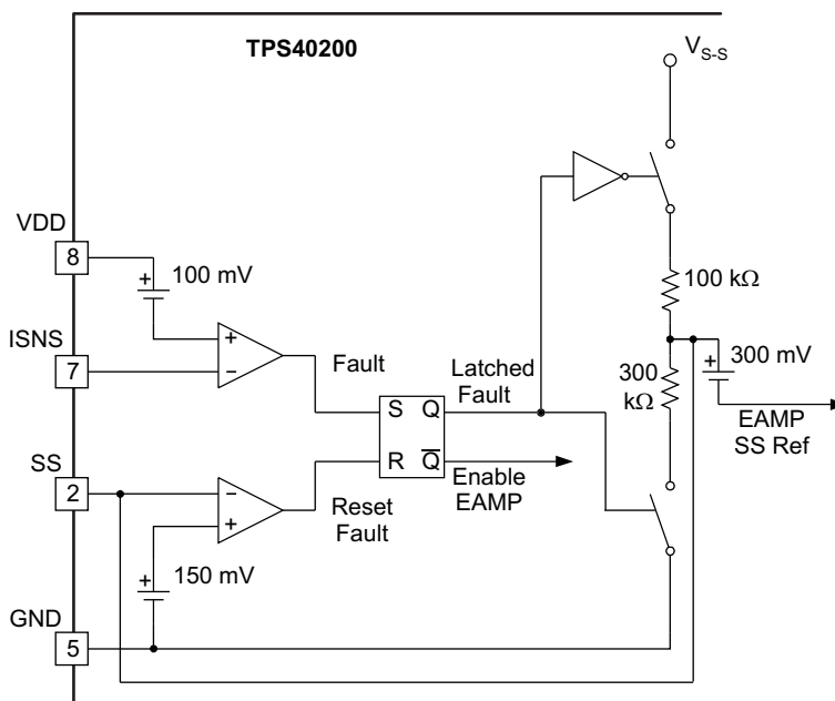
Figure 27. Current-Limit Reset
