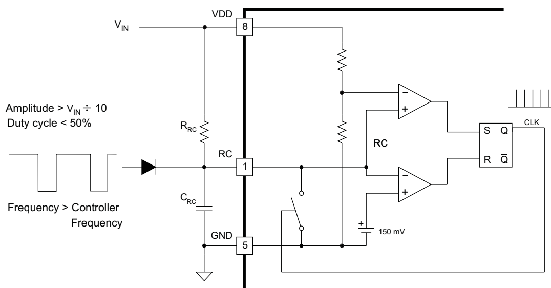
Figure 25. Diode-Connected Synchronization
