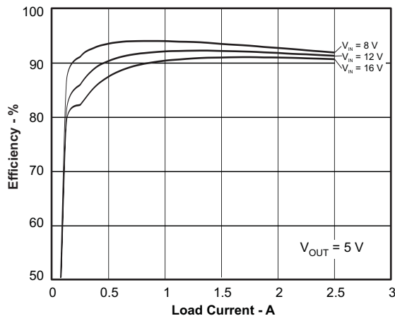
Figure 33. Full-Load Efficiency at 5-V V_{OUT}
