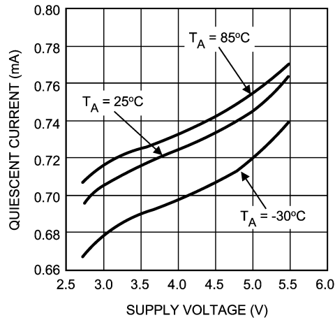
Quiescent Current vs Supply Voltage (V_{CON} = 0.267V, FB = 2V, \text{No load})
