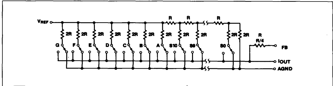
Figure 2. Simplified Circuit Diagram for the MX7538 D/A Section
