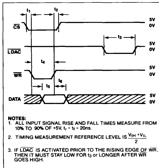
Figure 1. MX7538 Timing Diagram
