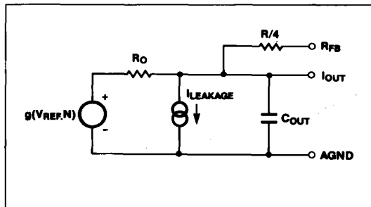
Figure 3. MX7538 Equivalent Analog Output Circuit
