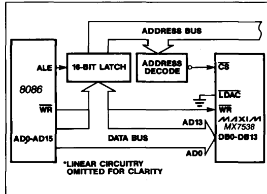
Figure 6. MX7538 - 8086 Interface Circuit
