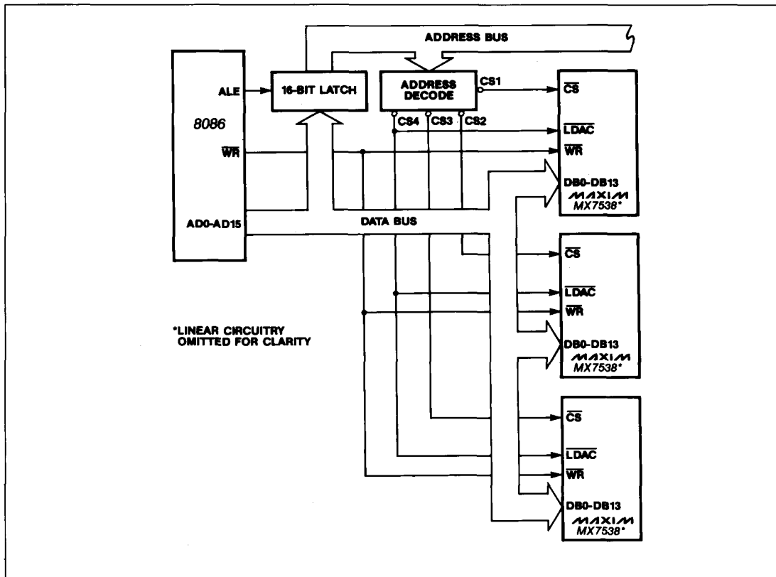
Figure 7. MX7538 - 8086 Interface: Multiple DAC System
