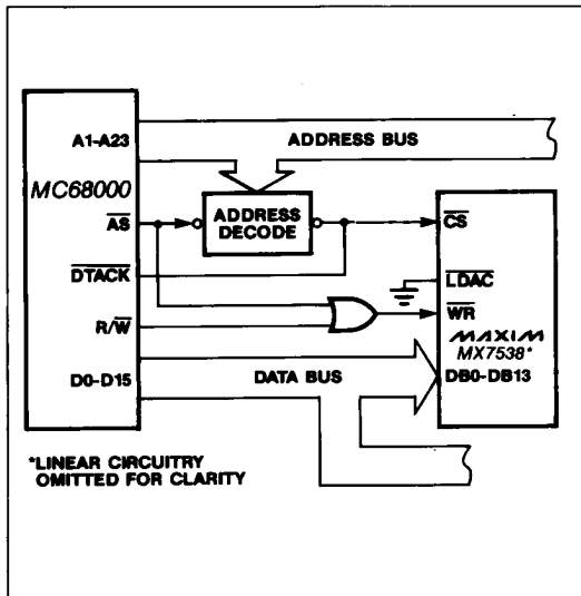
Figure 8. MX7538 - MC6800 Interface
