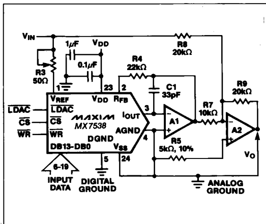
Figure 5. Bipolar Operation
