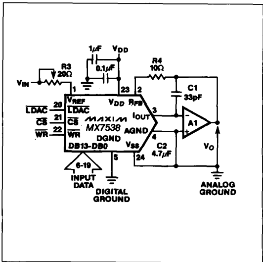
Figure 4. Unipolar Binary Operation
