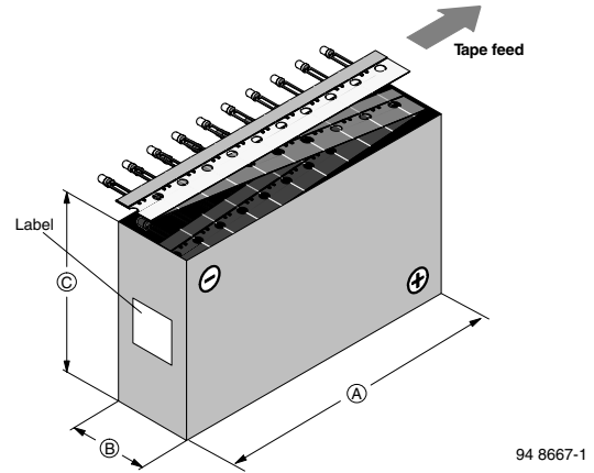
Figure 31. Tape Direction
