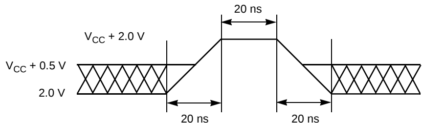
Figure 6. Maximum Positive Overshoot Waveform
