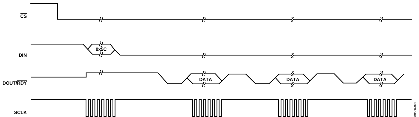
Figure 26. Continuous Read
