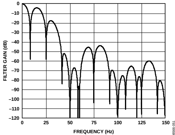
Figure 52. \text{Sinc}^3 Filter Response (FS[9:0] = 96, Chop Enabled, REJ60 = 1)
