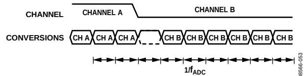
Figure 54. Fast Settling, \text{Sinc}^4 Filter
