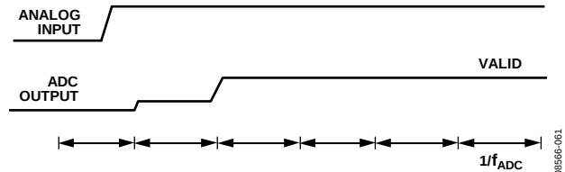
Figure 62. Step Change on Analog Input, Sinc 3 Filter
