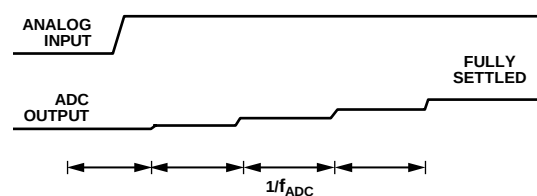
Figure 37. Asynchronous Step Change in Analog Input
