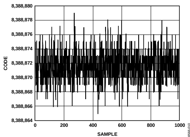
Figure 10. Noise ( V_{REF} = AV_{DD} = 5\text{ V} , Output Data Rate = 42.1 Hz (FS[9:0] = 6, Average by 16), Gain = 1, Chop Disabled, Sinc 4 Filter)
