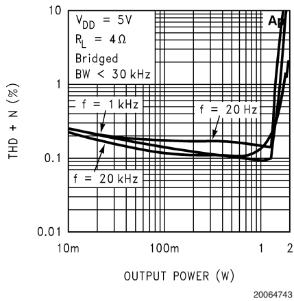
THD+N vs Output Power
