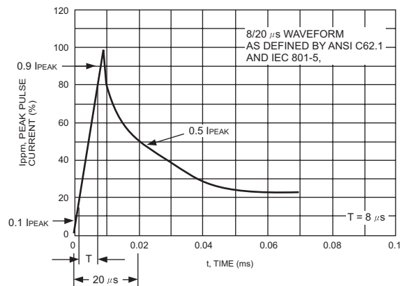
FIG.8- PULSE WAVEFORM
