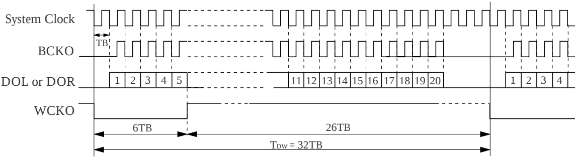
Figure 10. 8fs data output timing ( \overline{\text{CKSL}} = \text{LOW} )
