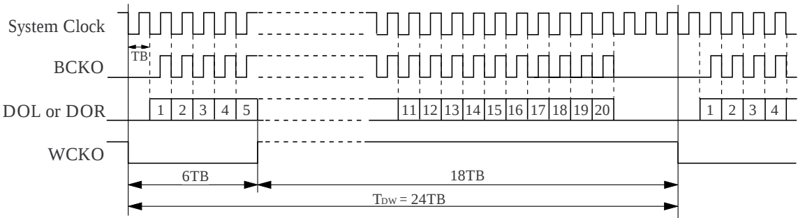
Figure 9. 8fs data output timing ( \overline{\text{CKSL}} = \text{HIGH} )
