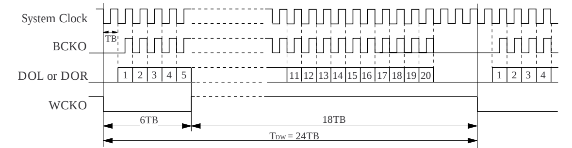
Figure 4. 8fs data output timing ( \overline{\text{CKSL}} = \text{HIGH} )
