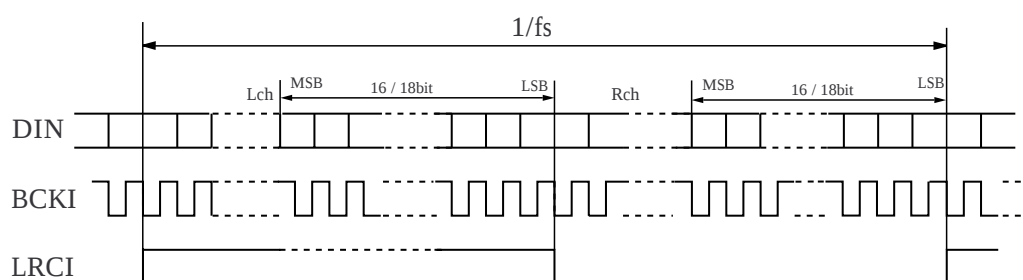
Figure 3. Audio data input timing
