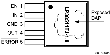
Top View TO-263 THIN 5 Pin Package
