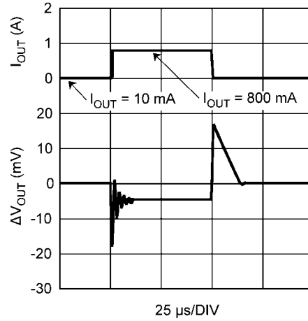
Load Transient, 10 mA to 800 mA C_{OUT} = 10 \mu F Ceramic
