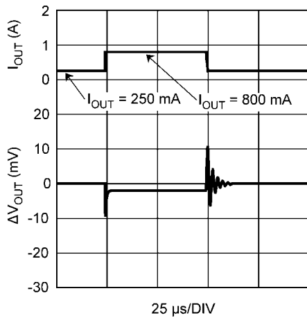
Load Transient, 250 mA to 800 mA C_{OUT} = 10 \mu F Ceramic + 100 \mu F Aluminum
