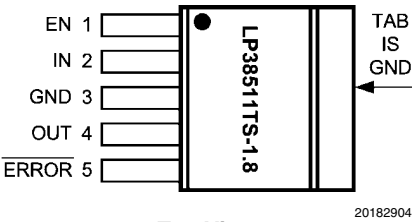
Top View TO-263 5 Pin Package
