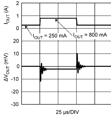
Load Transient, 250 mA to 800 mA C_{OUT} = 10 \mu F Ceramic
