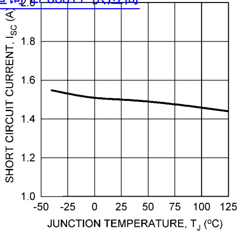
Current Limit vs Temperature 查询LP38511"供应商
