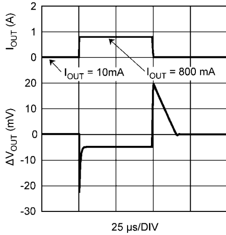
Load Transient, 10 mA to 800 mA C_{OUT} = 10 \mu F Ceramic + 100 \mu F Aluminum
