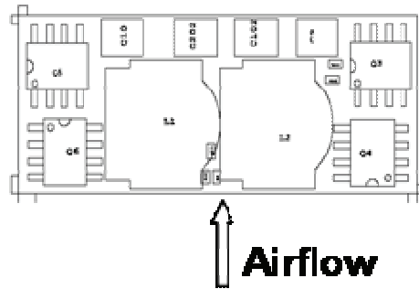
Figure 55. Airflow direction for thermal testing.
