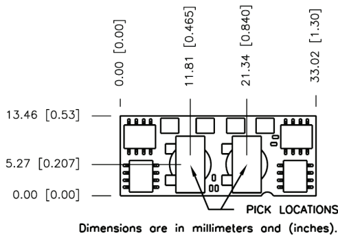
Figure 57. Pick and Place Location.
