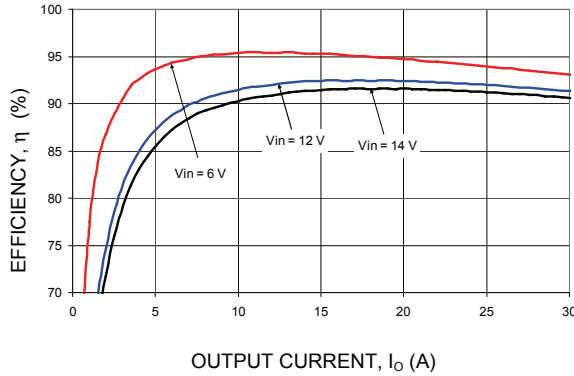
Figure 16. Converter Efficiency versus Output Current.
