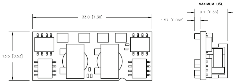
TOP VIEW
