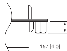
SL Option Bottom side riveted #4-40 Clinch Nuts
