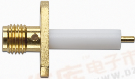
Model 72961 SMA JACK PANEL RECEPTACLE (2 HOLE)
