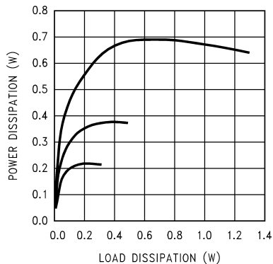
Power Dissipation vs Load Dissipation
