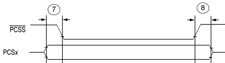
Figure 36. DSPI PCS Strobe ( \overline{\text{PCSS}} ) Timing
