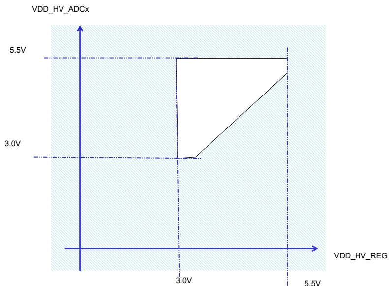
Figure 7. Independent ADC supply
