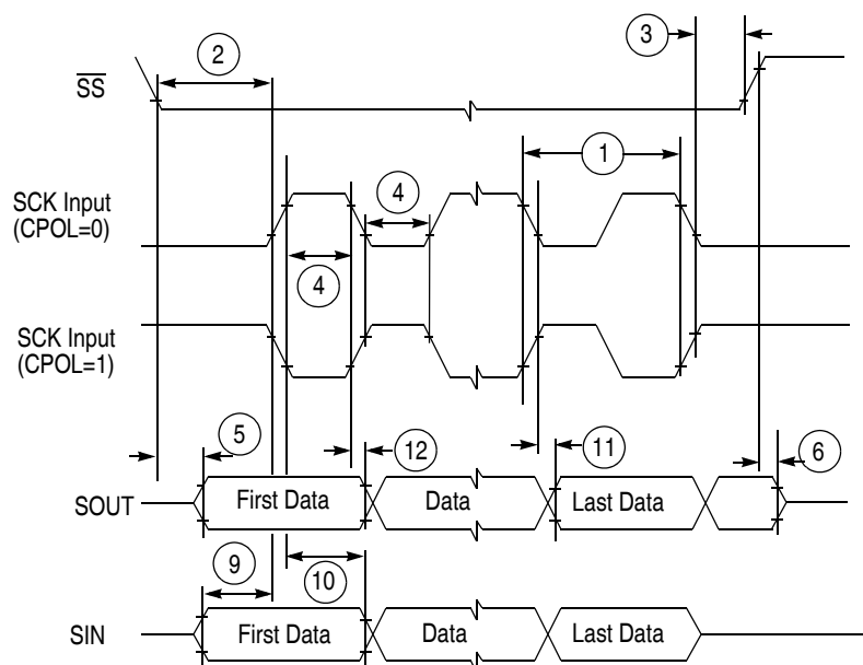
Figure 30. DSPI Classic SPI Timing - Slave, CPHA = 0
