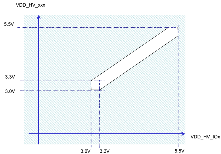
Figure 6. Power supplies constraints 1
