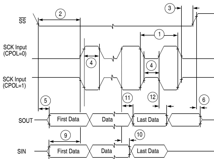
Figure 34. DSPI Modified Transfer Format Timing - Slave, CPHA = 0
