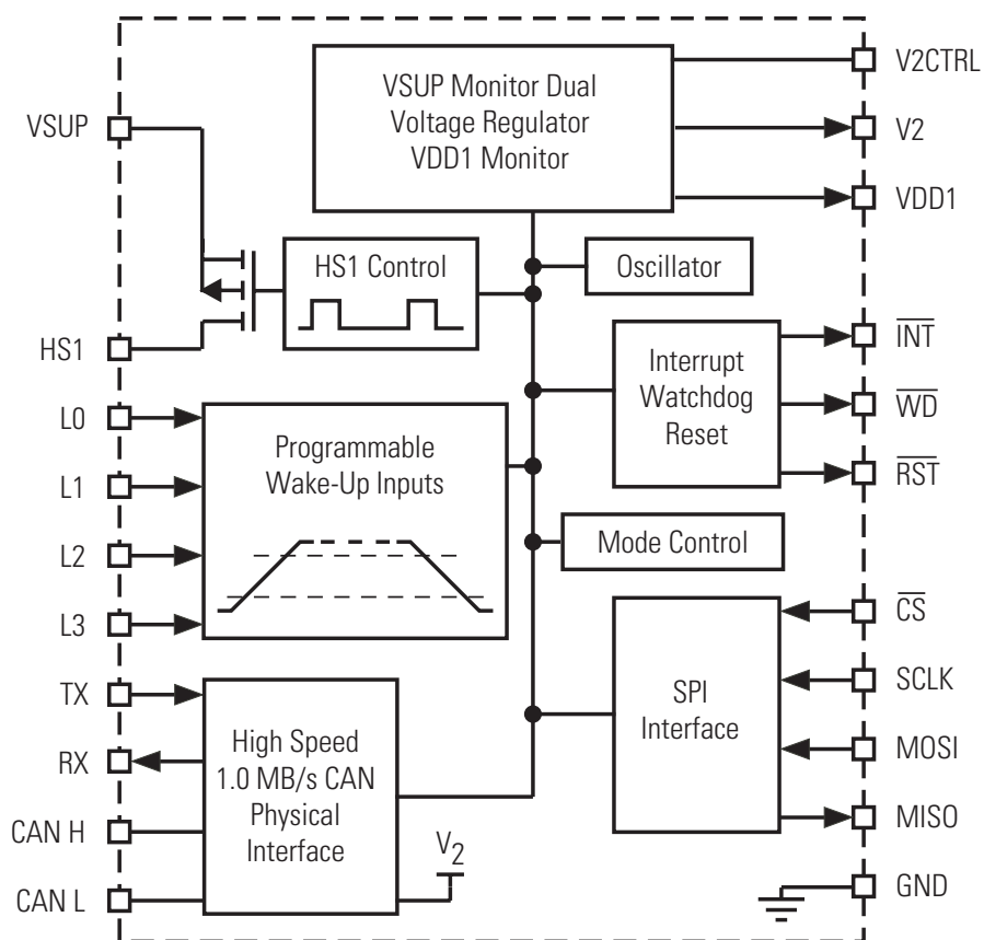
Figure 2. 33989 Simplified Internal Block Diagram
