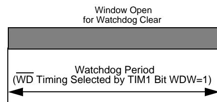
Figure 18. Timeout Watchdog
