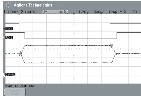
CAN signal with slew rate 3 selected
