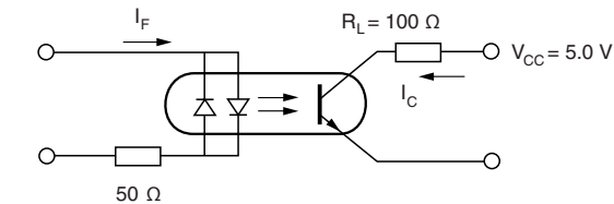
Fig. 1 - Linear Operation (without Saturation)
