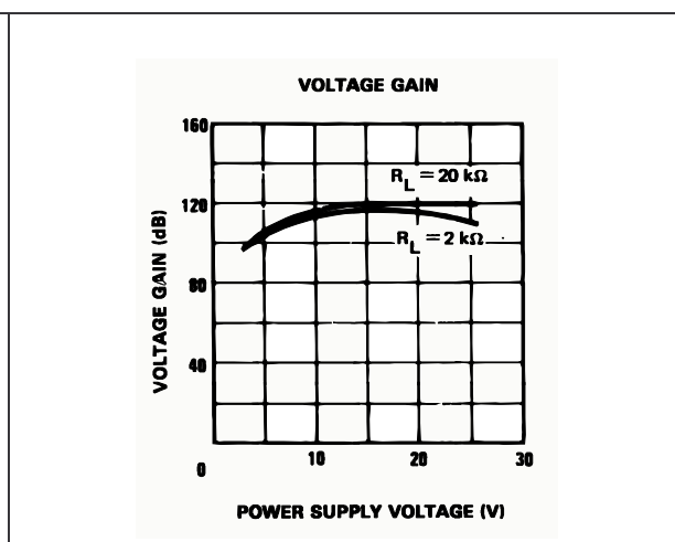
Figure 13. Voltage gain
