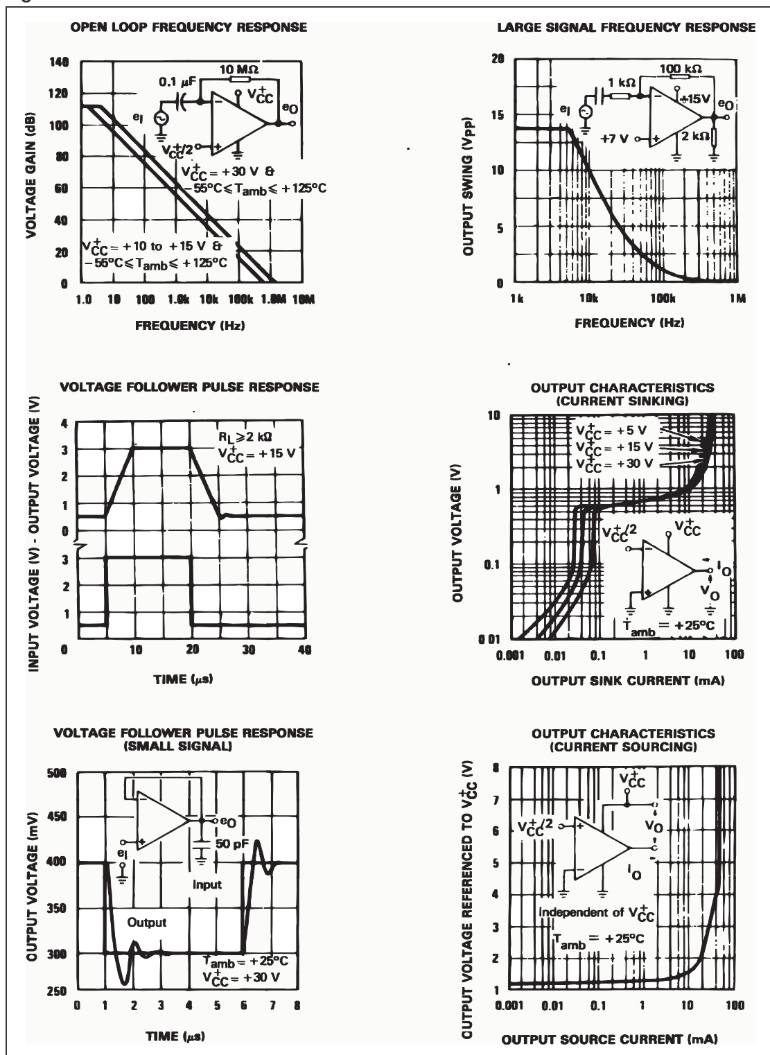
Figure 9. Electrical curves
