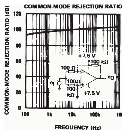
Figure 8. Common mode rejection ratio
