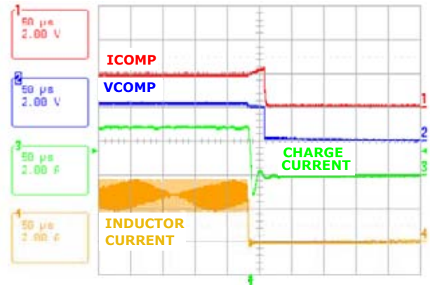
FIGURE 10. CHARGE DISABLE
