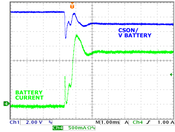
FIGURE 14. BATTERY INSERTION
