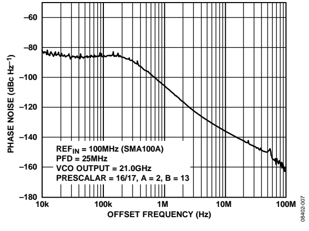
Figure 7. Phase Noise Plot of 20 GHz PLL Output Using the ADF5001 Prescaler and ADF4106 Synthesizer ICs
