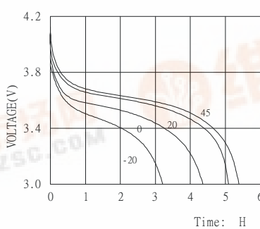
DISCHARGE CURVE AT VARIOUS TEMPERATURES(12mA)
