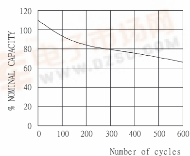
CYCLE LIFE CURVE
