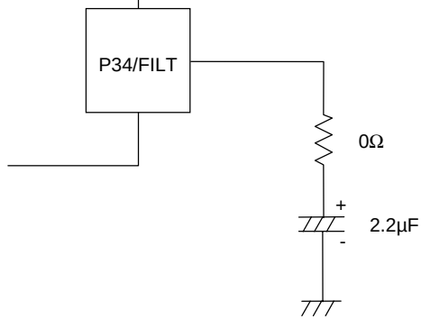
Figure 5 Filter Circuit for the Internal PLL Circuit
