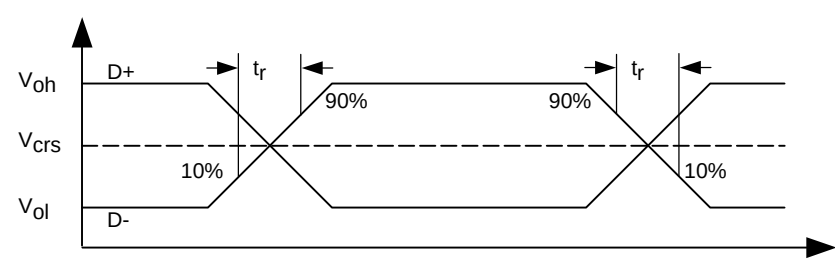
Figure 10 USB Data Signal Timing and Voltage Level
