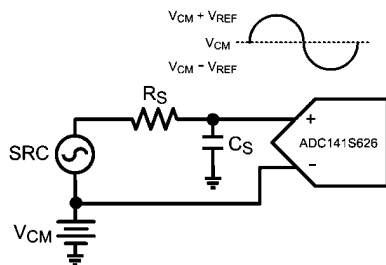
FIGURE 10. Single-Ended Input
