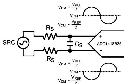
FIGURE 9. Differential Input
