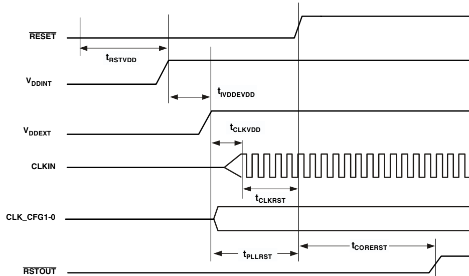
Figure 7. Power-Up Sequencing
