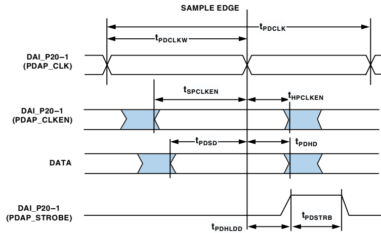
Figure 25. PDAP Timing
