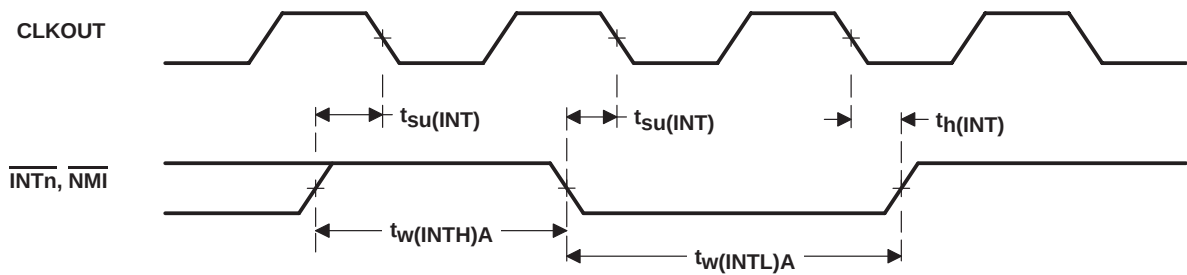
Figure 25. Interrupt Timing
