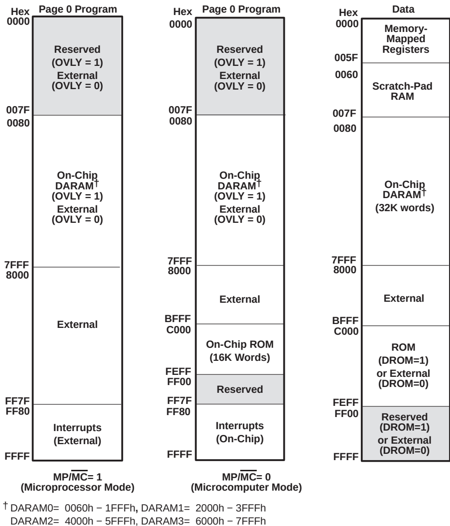
Figure 1. Memory Map
