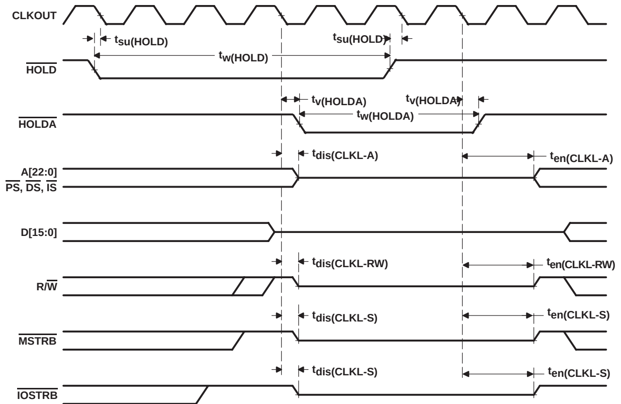
Figure 23. \overline{\text{HOLD}} and \overline{\text{HOLDA}} Timings (HM = 1)
