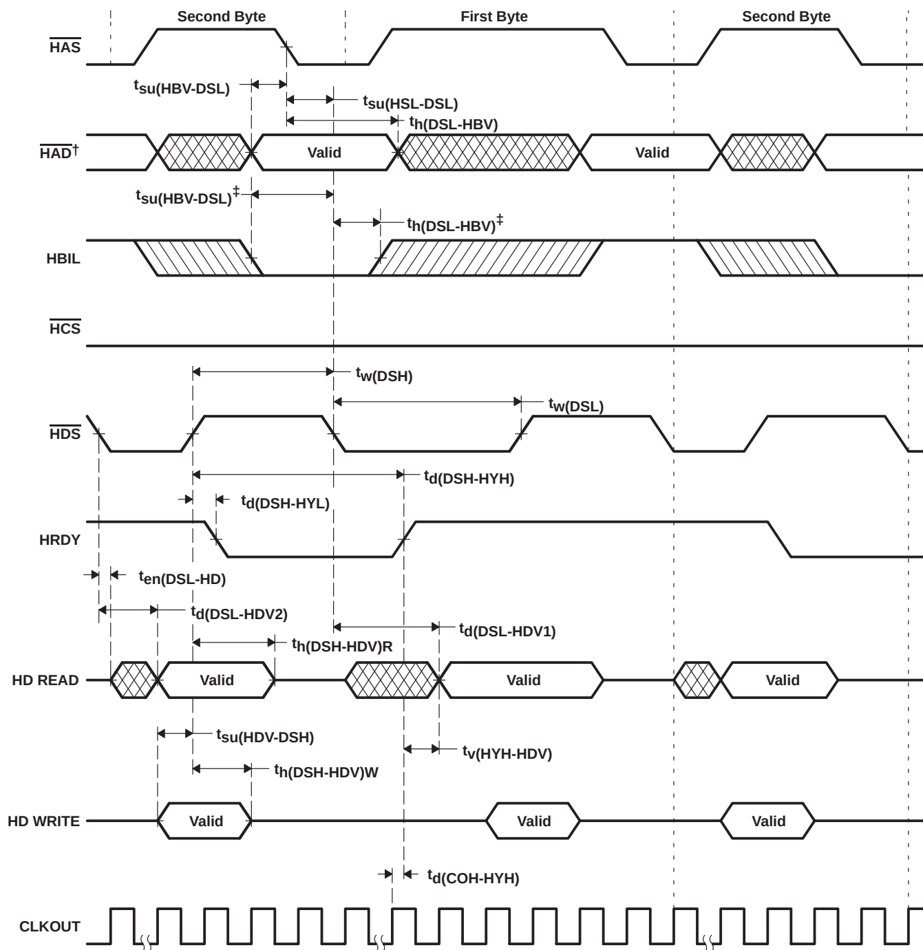
Figure 37. Using \overline{\text{HDS}} to Control Accesses ( \overline{\text{HCS}} Always Low)
