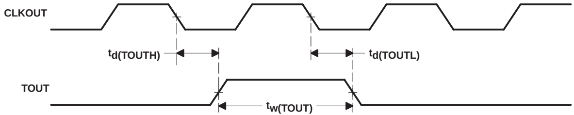
Figure 29. TOUT Timing
