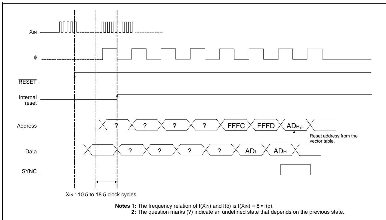
Fig 61. Reset sequence
