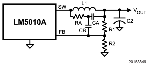
FIGURE 11. Low Output Ripple Using Ripple Injection
