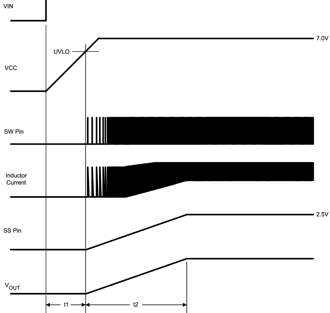
FIGURE 1. Startup Sequence
