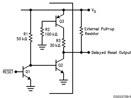
FIGURE 1. Delay Reset Output
