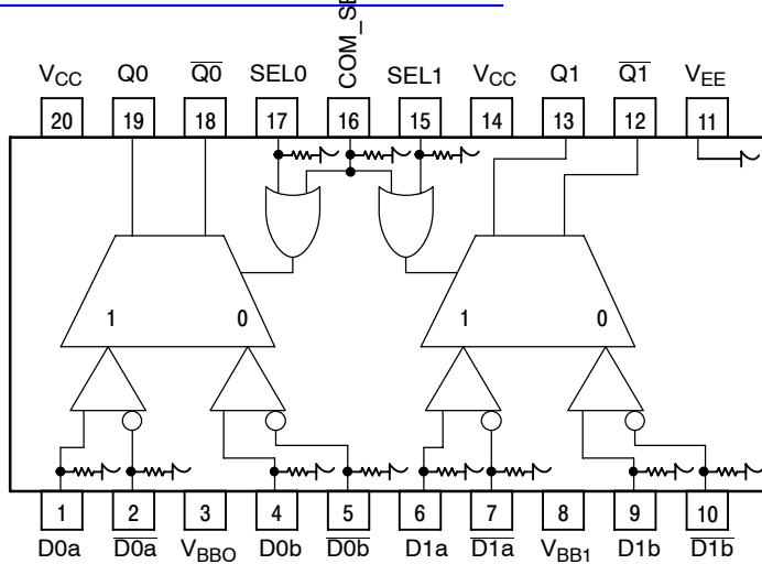
Figure 1. 20-Lead Package (Top View) and Logic Diagram
