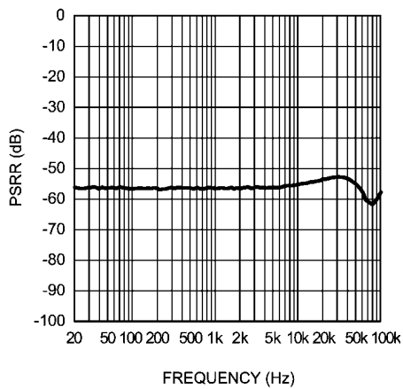
Earpiece PSRR vs Frequency V_{DD} = 3.3V , 0dB DAC (DAC input selected)
