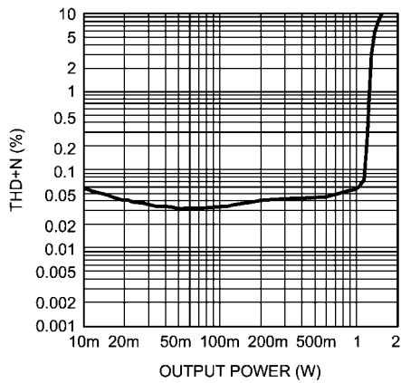
Loudspeaker THD+N vs Output Power AV_{DD} = 5V, 0dB\ CPI f_{OUT} = 1kHz, 15\mu H + 8\Omega + 15\mu H
