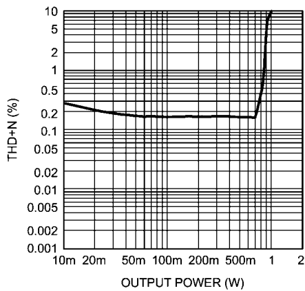
Loudspeaker THD+N vs Output Power AV_{DD} = 4.2V, 0dB\ DAC f_{OUT} = 1kHz, 15\mu H + 8\Omega + 15\mu H
