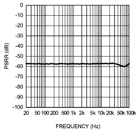
Earpiece PSRR vs Frequency V_{DD} = 5V , 0dB DAC (DAC input selected)
