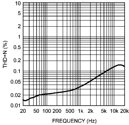
查询"LM49370"供应商 Earpiece THD+N vs Frequency AV_{DD} = 5V, 0dB, P_{OUT} = 50mW, 32\Omega
