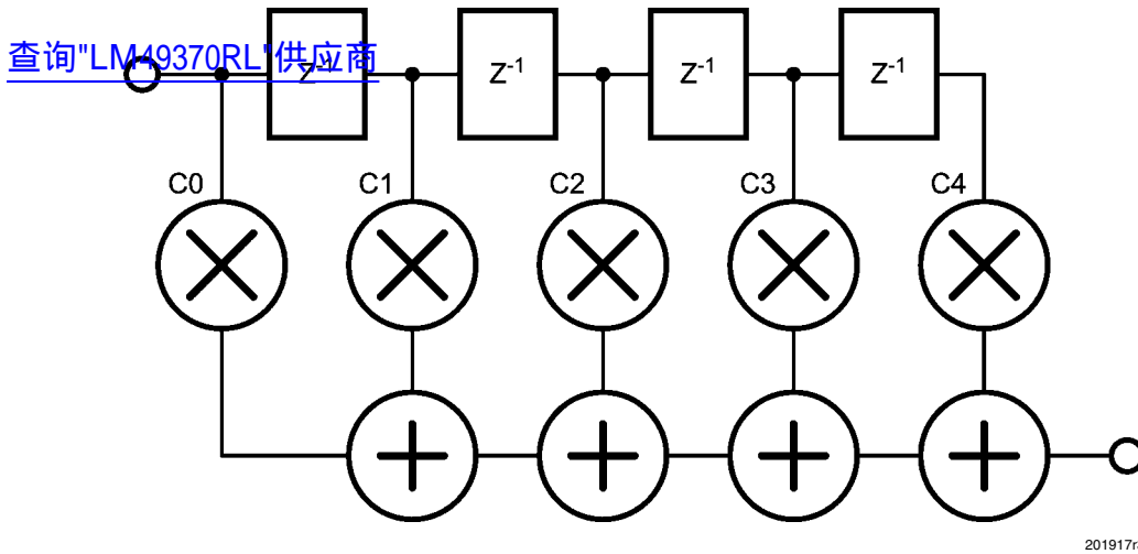
FIGURE 15. FIR Consumption Filter Taps
