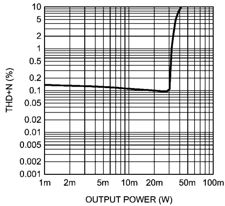
Headphone THD+N vs Output Power AV_{DD} = 5V, OCL, 0dB\ AUX f_{OUT} = 1kHz, 32\Omega
