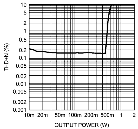
Loudspeaker THD+N vs Output Power AV_{DD} = 3.3V, 0dB\ DAC f_{OUT} = 1kHz, 15\mu H + 8\Omega + 15\mu H
