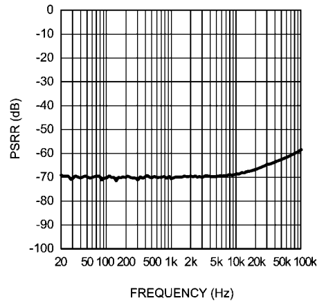
Earpiece PSRR vs Frequency V_{DD} = 5V , 0dB CPI (CPI input terminated)
