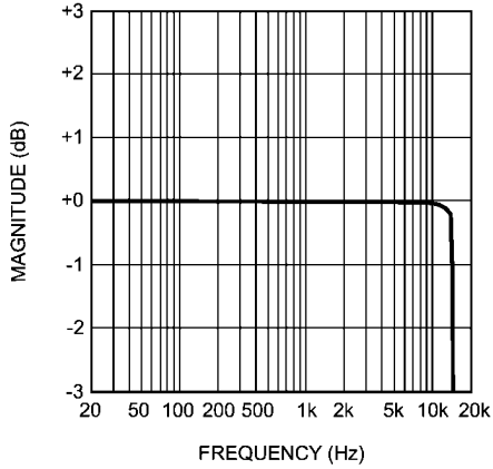
查询"LM49370"供应商 Stereo DAC Frequency Response f_s = 32\text{kHz}
