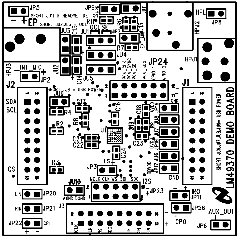
Top Silkscreen
