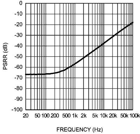
INT/EXT MICBIAS PSRR vs Frequency 查询"LM49370" datasheet AV_{DD} = 3.3V, MICBIAS = 2.0V
