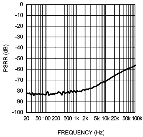
Earpiece PSRR vs Frequency V_{DD} = 3.3V , 0dB CPI (CPI input terminated)
