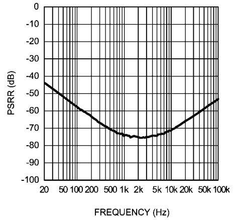
Earpiece PSRR vs Frequency V_{DD} = 5V , 0dB AUX (AUX inputs terminated)
