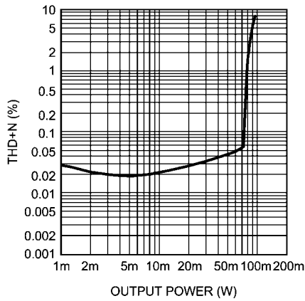
Headphone THD+N vs Output Power AV_{DD} = 5V, 0dB\ CPI f_{OUT} = 1kHz, 32\Omega
