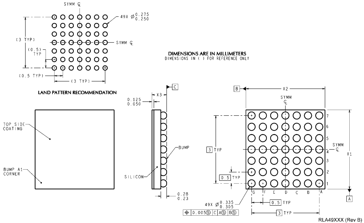
49 Bump micro SMDxt Package Order Number LM49370RL Dimensions: X1 = 3.924±0.03mm, X2 = 3.924±0.03mm, X3 = 0.650±0.75mm NS Package Number RLA49UUA
