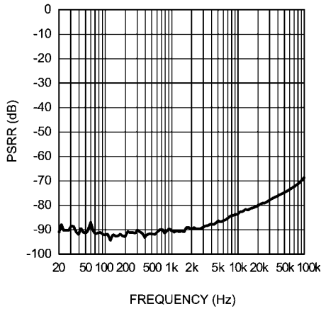
查询"LM49370"供应信息 AUXOUT PSRR vs Frequency AV_{DD} = 3.3V, 0dB DAC (DAC inputs selected)
