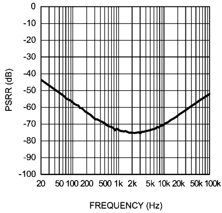
Earpiece PSRR vs Frequency V_{DD} = 3.3V , 0dB AUX (AUX inputs terminated)
