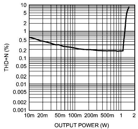
Loudspeaker THD+N vs Output Power AV_{DD} = 5V, 0dB\ DAC f_{OUT} = 1kHz, 15\mu H + 8\Omega + 15\mu H
