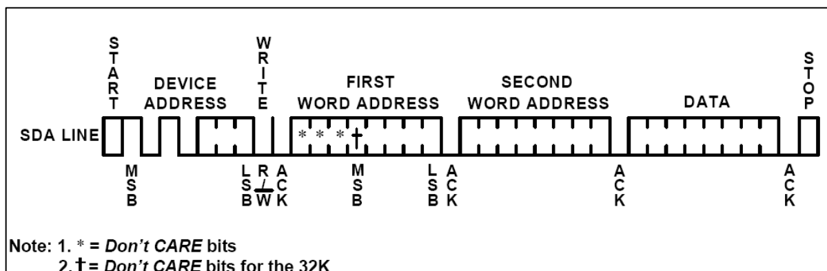
Figure 8 · Byte Write
