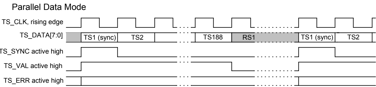
Figure 7. MPEG-TS Parallel Mode
