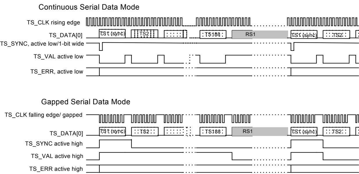
Figure 8. MPEG-TS Serial Modes
