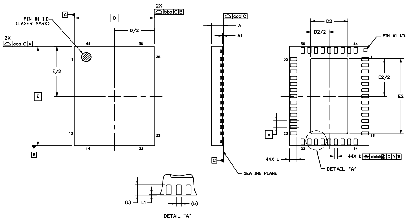
Figure 18. 44-Pin QFN
