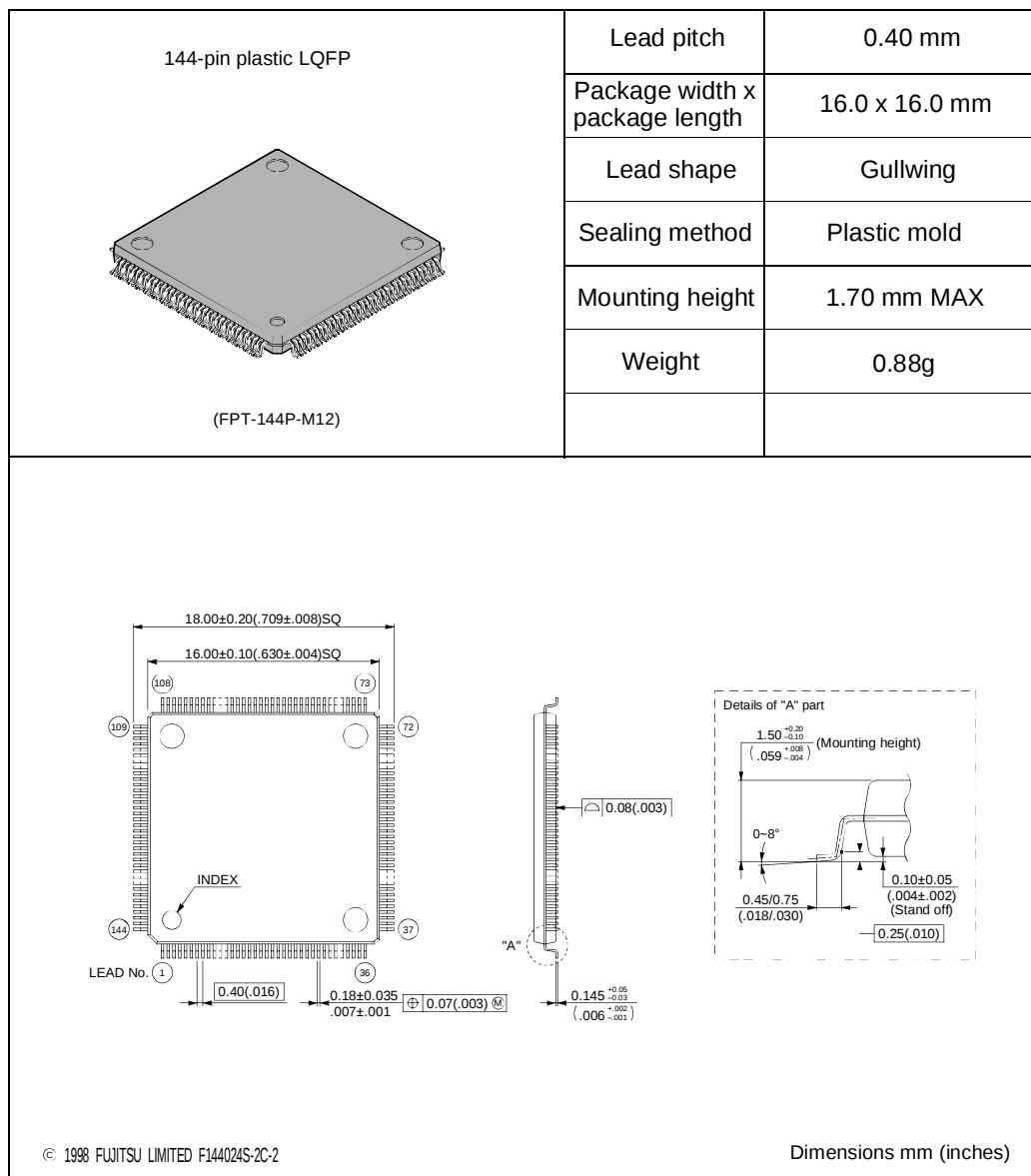
144-pin plastic LQFP (FPT-144P-M12)
