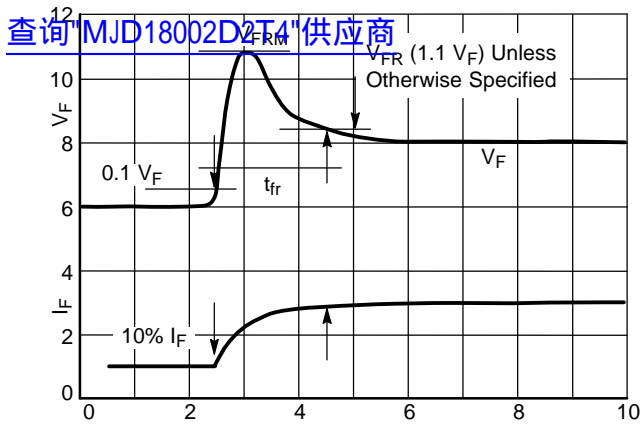
Figure 26. t_{fr} Measurement
