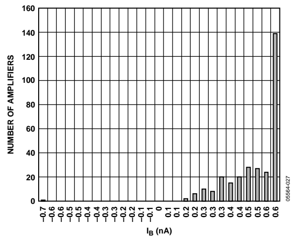
Figure 8. Input Bias Current, V SV = ±5 V
