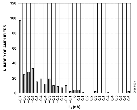
Figure 7. Input Bias Current, V SV = ±15 V
