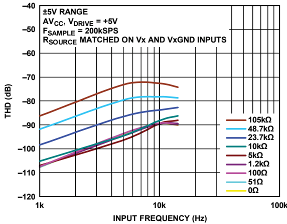
Figure 25. THD vs. Input Frequency for Various Source Impedances, ±5 V Range
