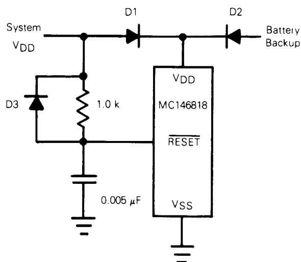
查询"MC146818D"供应商 FIGURE 13 — TYPICAL POWERUP DELAY CIRCUIT FOR RESET
