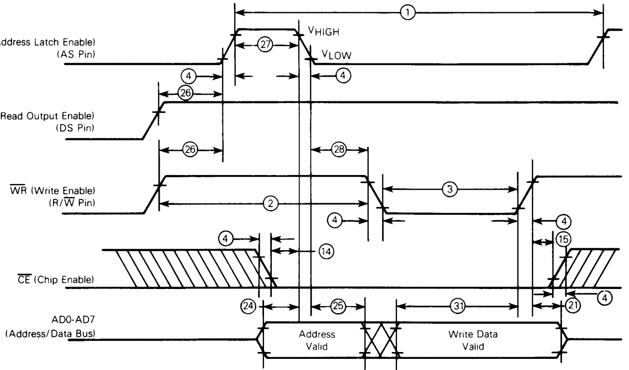
FIGURE 4 — BUS WRITE TIMING COMPETITOR MULTIPLEXED BUS
