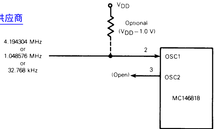
FIGURE 10 — EXTERNAL TIME-BASE CONNECTION
