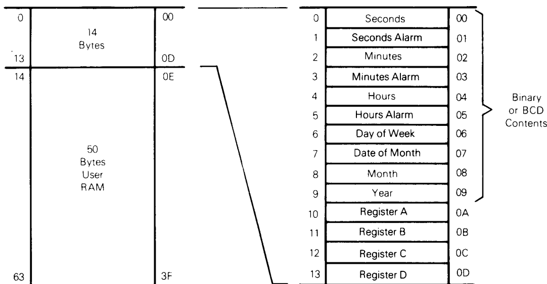
FIGURE 15 — ADDRESS MAP
