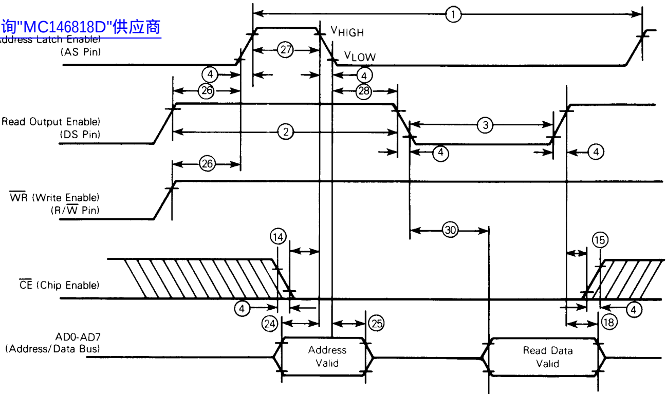
FIGURE 3 — BUS READ TIMING COMPETITOR MULTIPLEXED BUS
